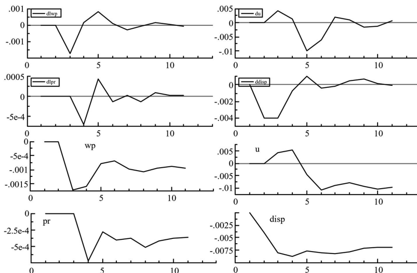
A RESPONSE TO AN IMPULSE IN \Delta pq
